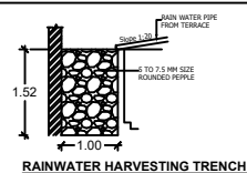
RAINWATER HARVESTING TRENCH
