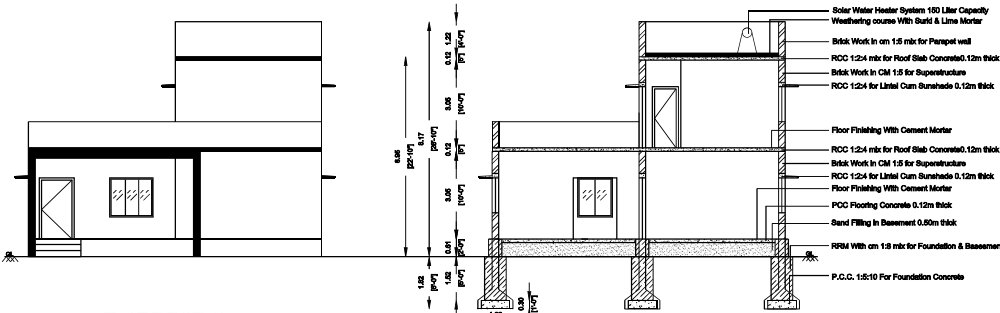
FRONT ELEVATION
