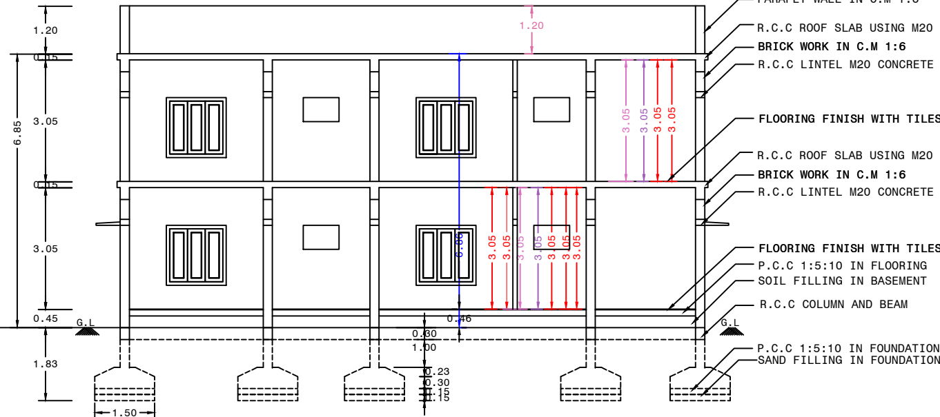
SECTION ON DD'
