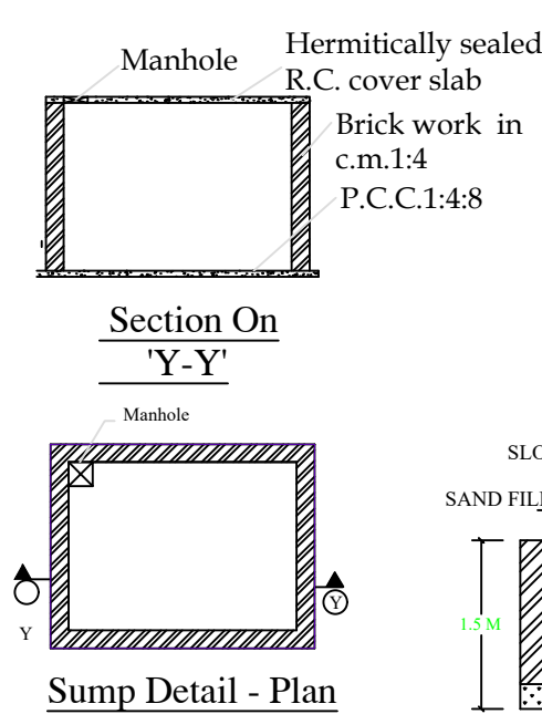
Sump Detail - Plan
