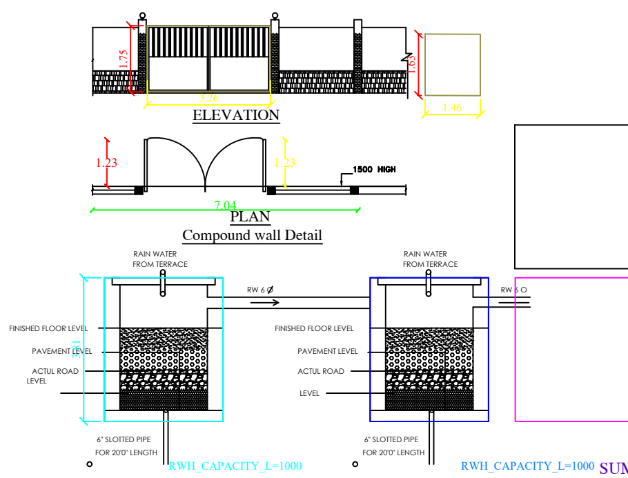
RAINWATER HARVESTING
