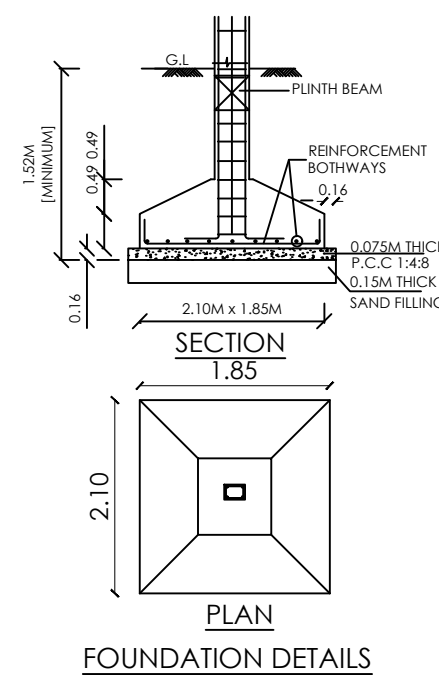
FOUNDATION DETAILS
