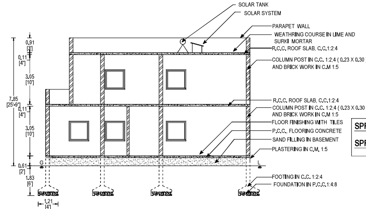
SECTION ON " S P "
