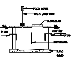
SEC. OF SEPTIC TANK
