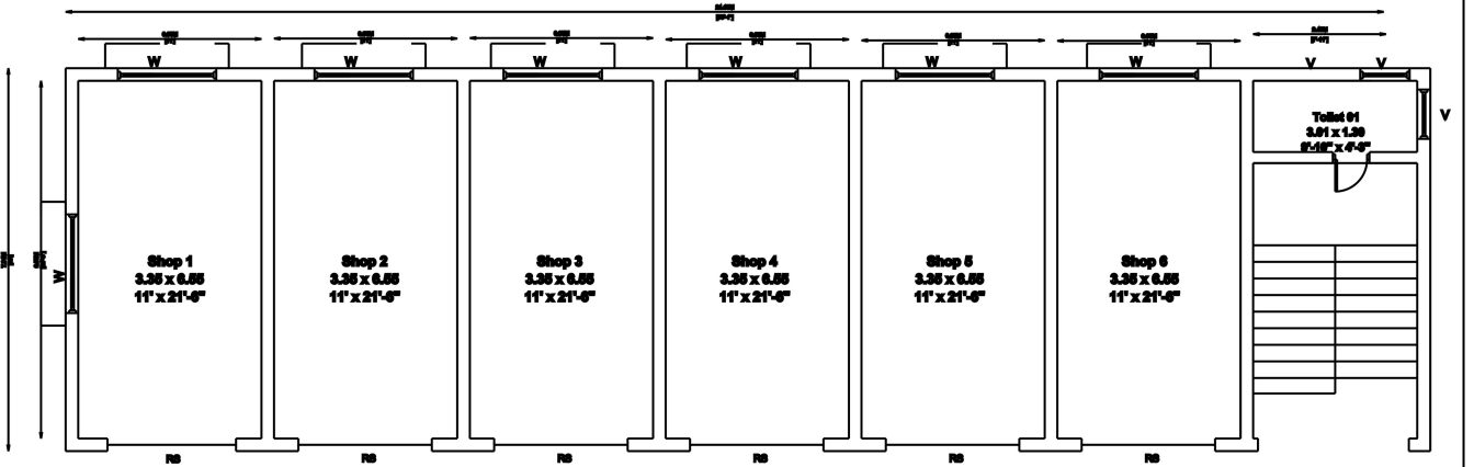
SITE CUM PRO.GROUND FLOOR
