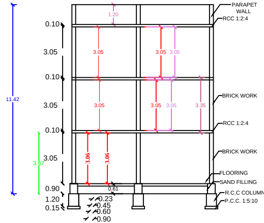
SECTION AB
