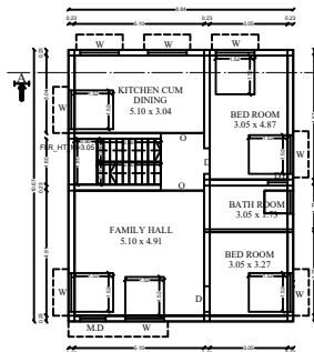
GROUND FLOOR PLAN SCALE-1:100
