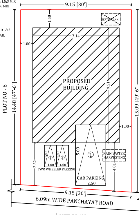
SITE PLAN
