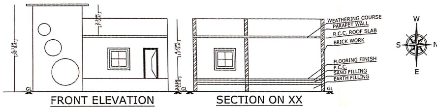
FRONT ELEVATION
