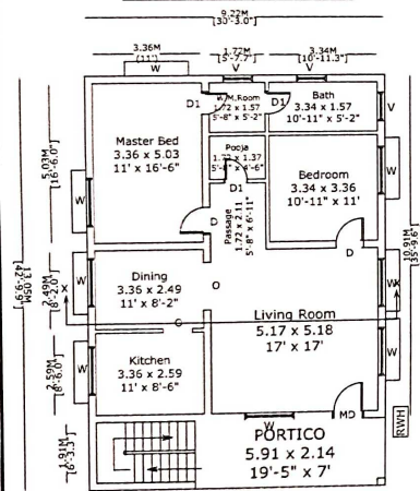
SITE CUM PRO.GROUND FLOOR
