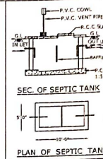
PLAN OF SEPTIC TANK
