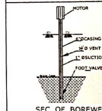
SEC. OF BOREWELL
