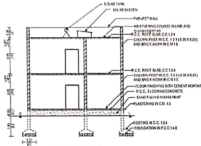
SECTION ON "S P"
