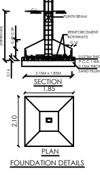
SECTION 1-2
