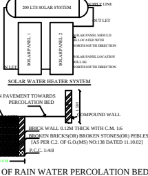
SECTION 1-2
