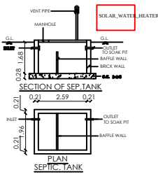
SECTION 1-2
