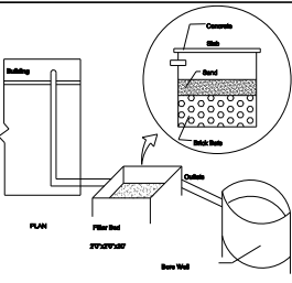
Rainwater Harvesting Tank
