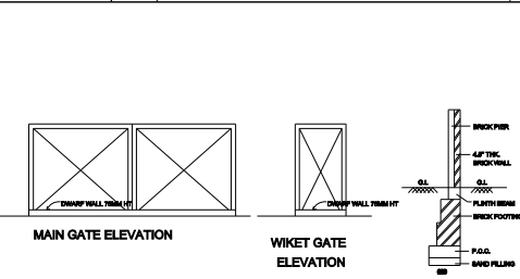
COMPOUND WALL DETAIL
