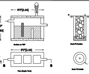
Septic Tank & Soak Pit Details
