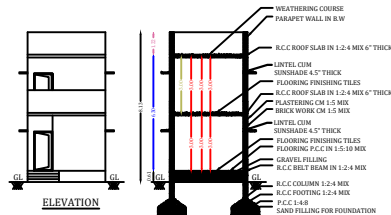
SECTION A TO B
