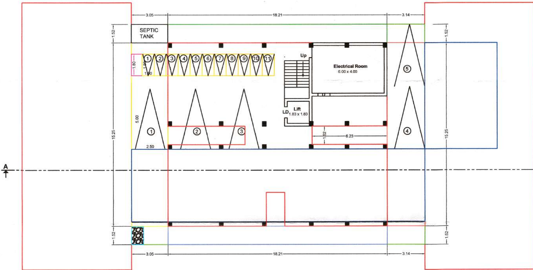
STILT FLOOR PLAN
