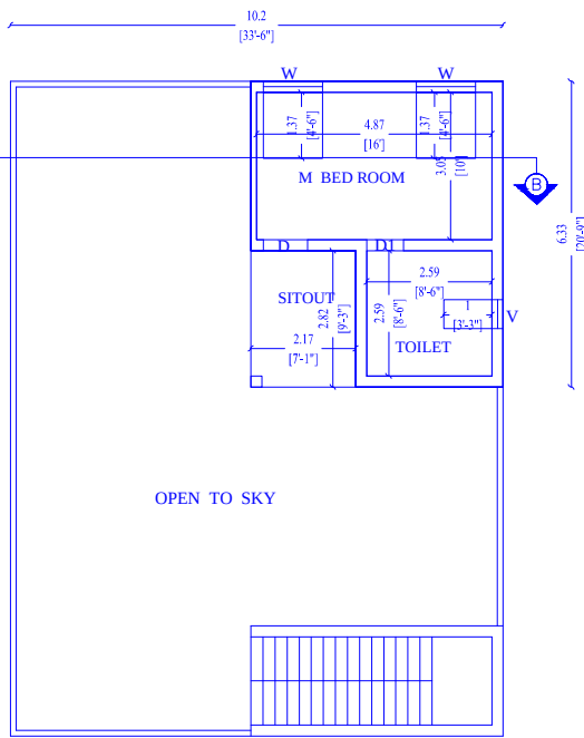
PLAN FOR FIRST FLOOR
