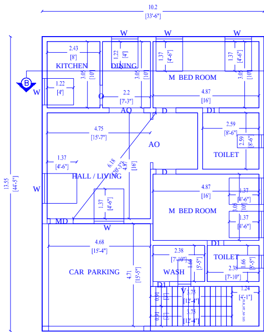
PLAN FOR GROUND FLOOR
