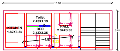
PROPOSED FIRST FLOOR PLAN
