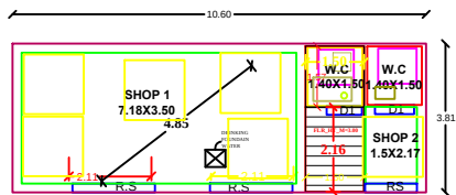
PROPOSED GROUND FLOOR PLAN
