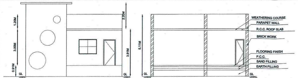
FRONT ELEVATION
