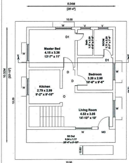
SITE CUM PRO.GROUND FLOOR
