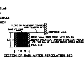
SECTION OF RAIN WATER PERCOLATION BED
