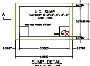
SUMP DETAIL SCALE 1" = 4'-0"
