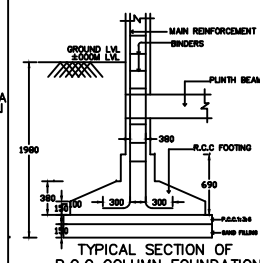
TYPICAL SECTION OF R.C.C COLUMN FOUNDATION SCALE : 1" = 2'-0"
