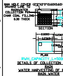
SECTION ON D-D
