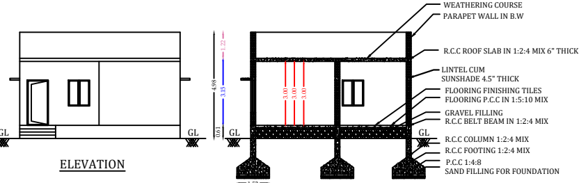
SECTION A TO B
