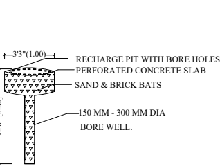
RAINWATER HARVESTING:-
