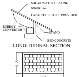
SOLAR SYSTEM
