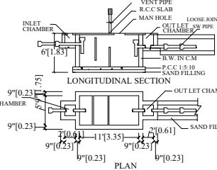
SEPTIC TANK:-
