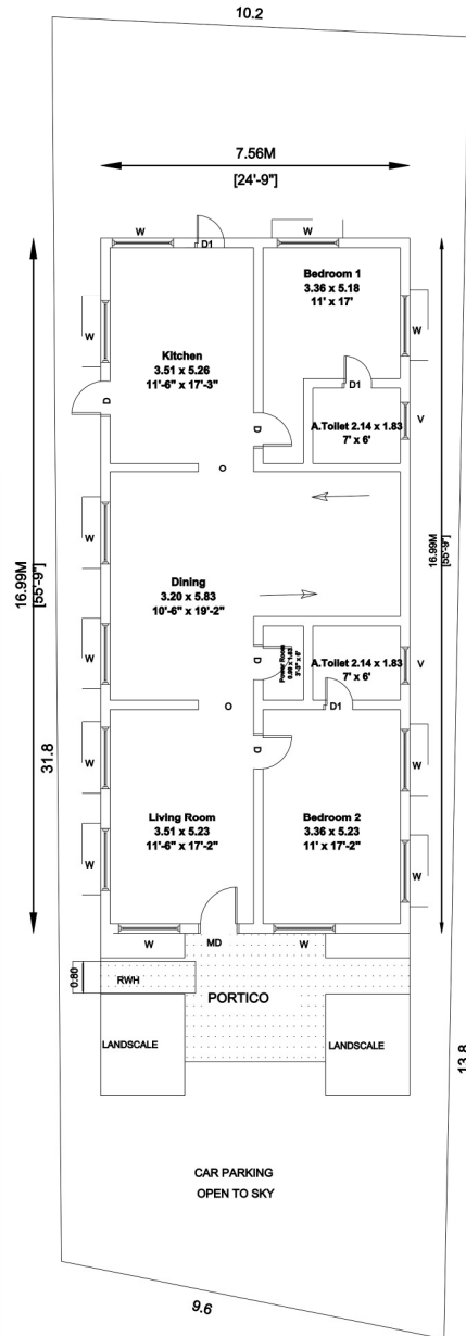
SITE CUM PRO.GROUND FLOOR
