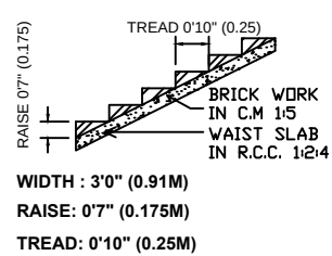
STAIR CASE DETAILS
