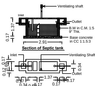
SEPTIC TANK DETAIL
