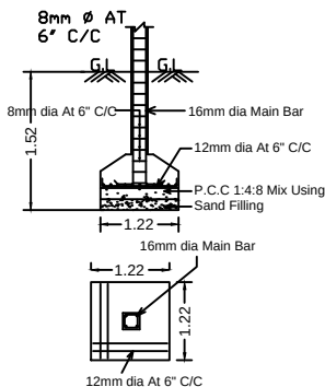
COLUMN SIZE - 9" X 12"
