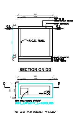
PLAN OF RWH TANK
