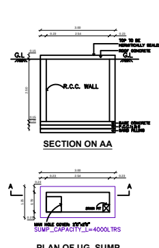
PLAN OF UG SUMP
