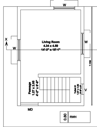
SITE CUM PRO.GROUND FLOOR
