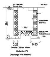
DETAILS OF RAIN WATER COLLECTION PE (Recharge Well Method) SCALE: 1"=4'0"
