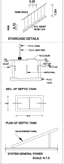
STAIRCASE DETAILS
