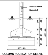
COLUMN FOUNDATION DETAIL
