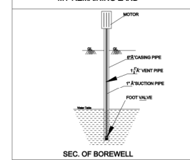
SEC. OF BOREWELL
