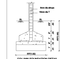
COLUMN FOUNDATION DETAIL
