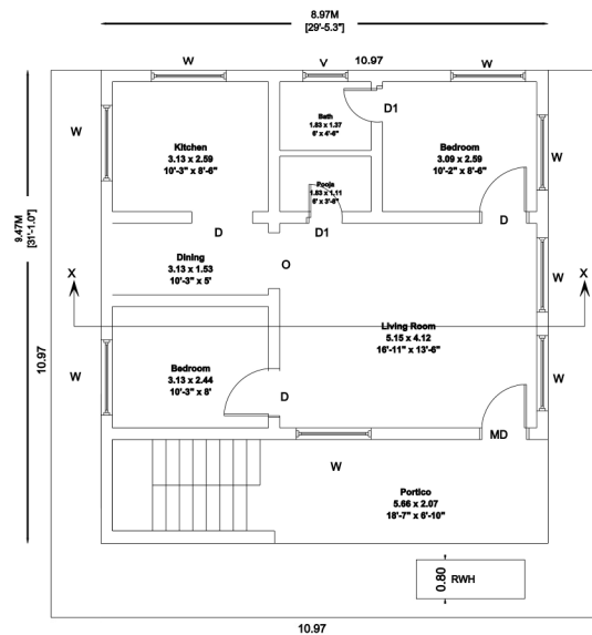
SITE CUM PRO.GROUND FLOOR
