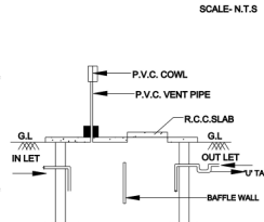
SEC. OF SEPTIC TANK
