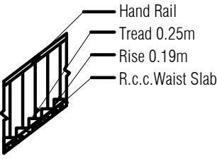
STAIR DETAILS
