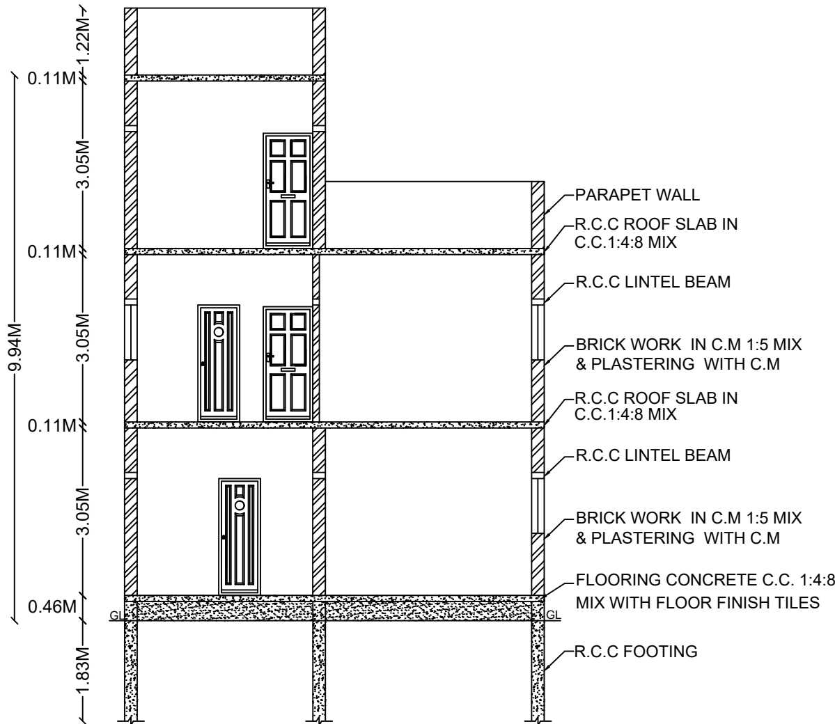
SECTION 'AA'
