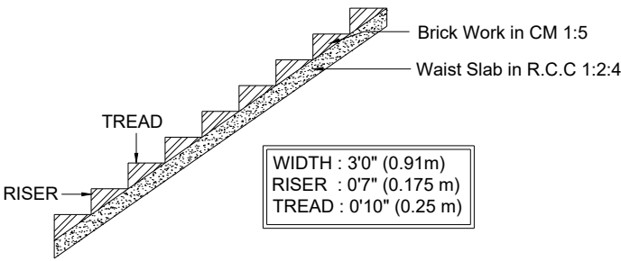
STAIRCASE DETAILS
