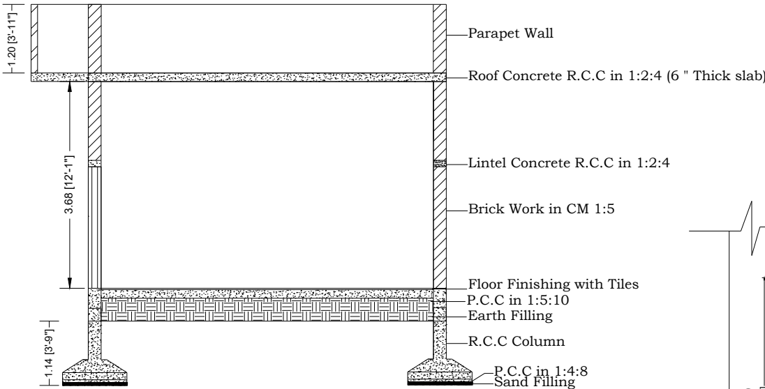
SECTION X-X
