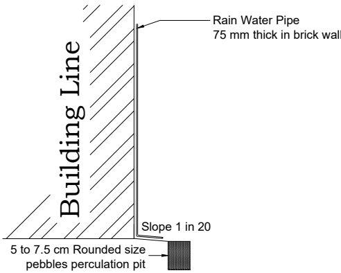
RAINWATER HARVESTING
