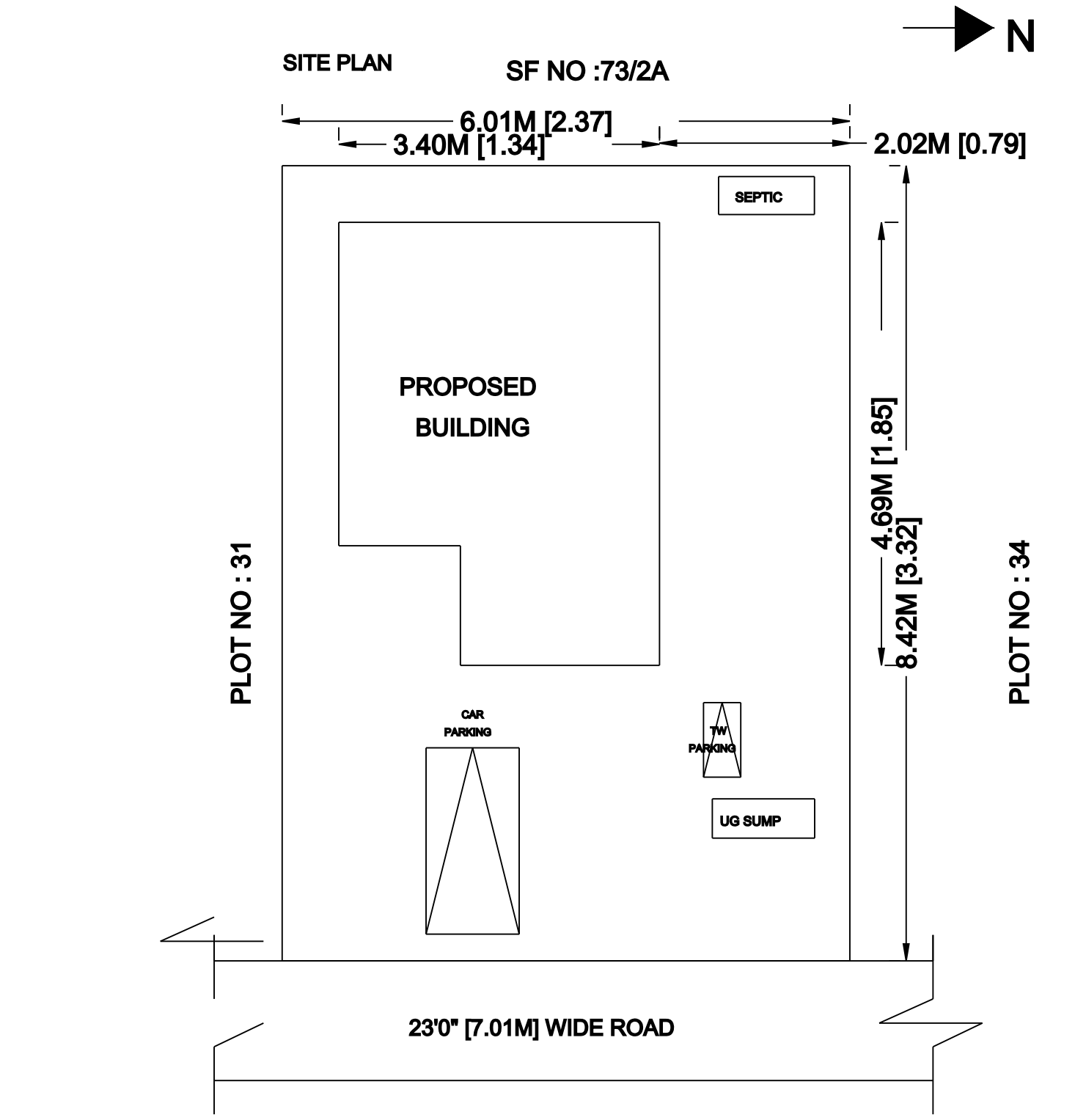
KEY PLAN
