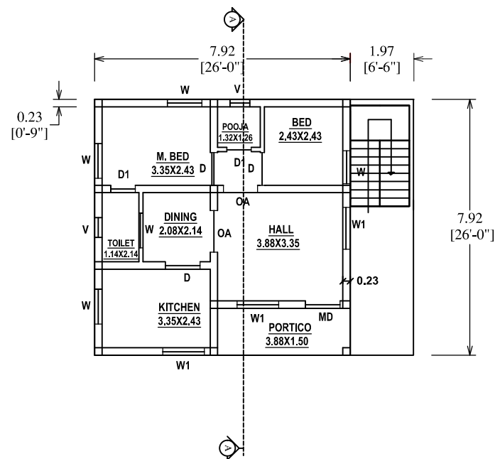
GROUND FLOOR PLAN FACED TO EAST
