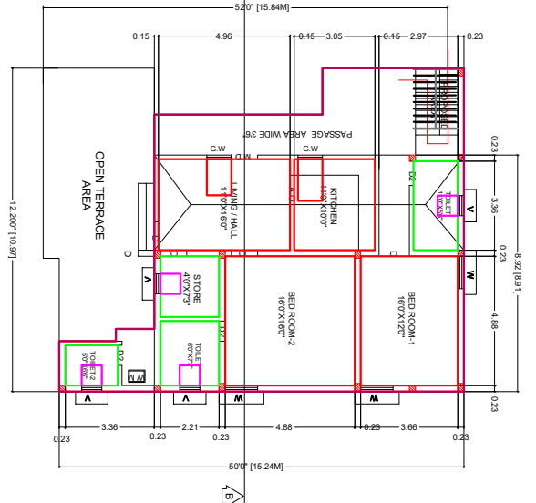
SECTION PLAN - "A-B"
