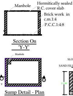
Sump Detail - Plan
