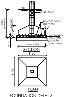
FOUNDATION DETAILS
