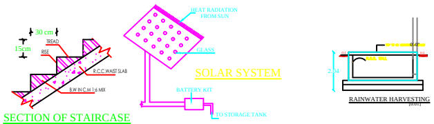
SECTION OF STAIRCASE
