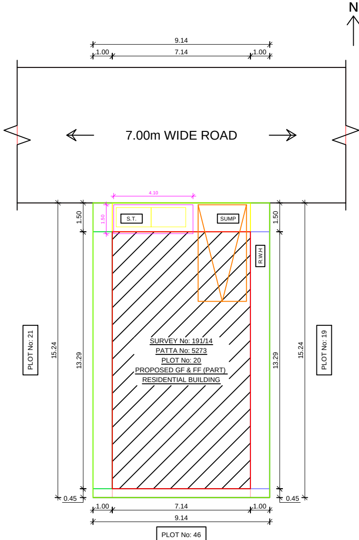
SITE PLAN
