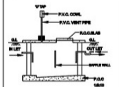
SEC. OF SEPTIC TANK
