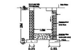
Details Of Rain Water
