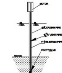
SEC. OF BOREWELL
