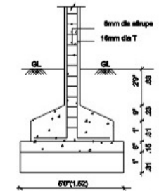
COLUMN FOUNDATION
