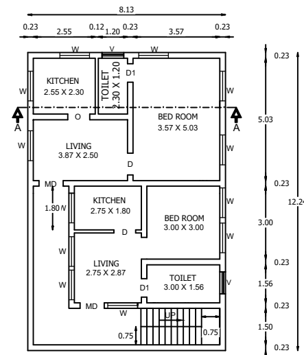
FLOOR 1ST & 2ND TYPICAL PLAN
