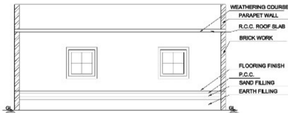
SECTION ON XX
