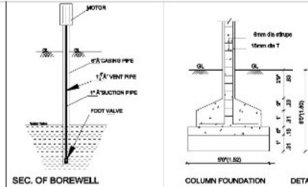
SEC. OF BOREWELL
