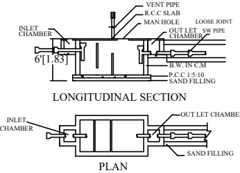
SEPTIC TANK:
