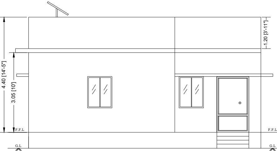
FRONT ELEVATION
