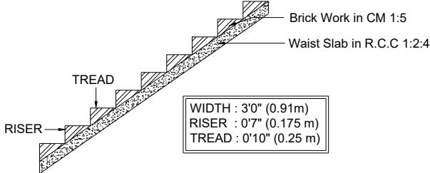
STAIRCASE DETAILS
