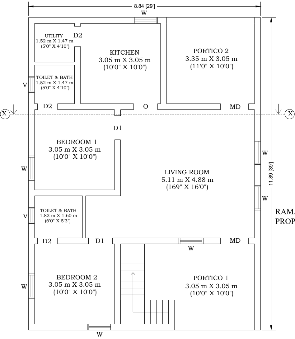
GROUND FLOOR
