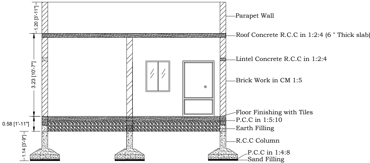
SECTION X-X
