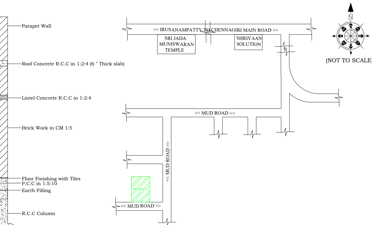
KEY PLAN
