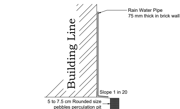
RAINWATER HARVESTING
