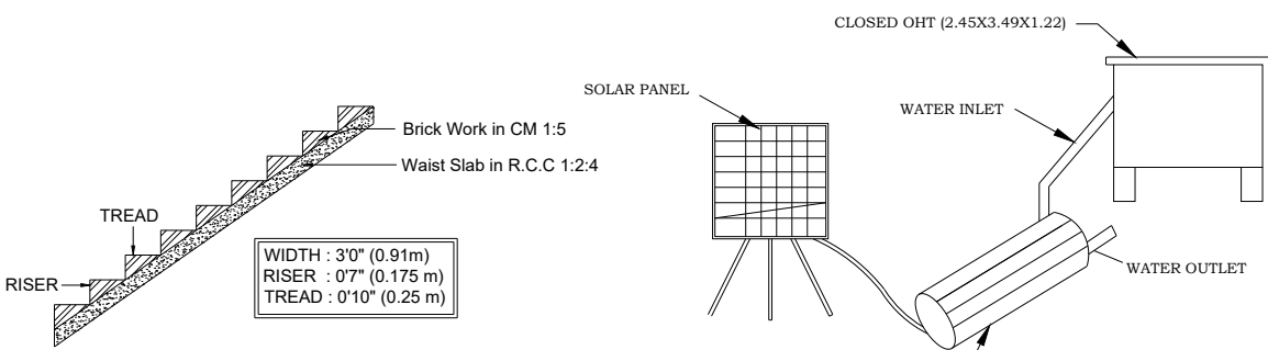
STAIRCASE DETAILS
