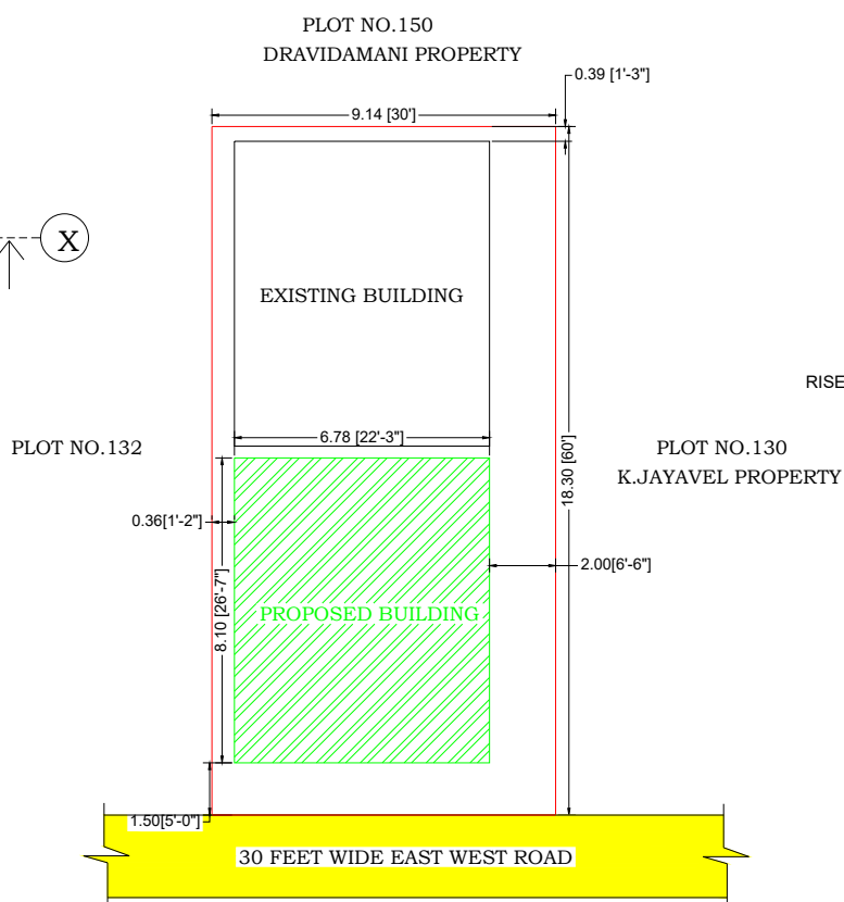
SITE PLAN
