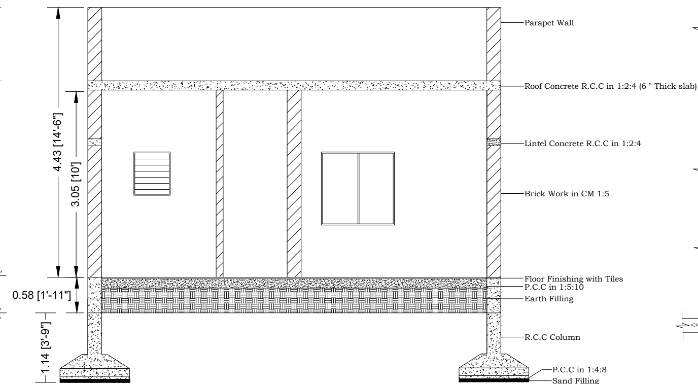
SECTION X-X
