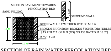
SECTION OF RAIN WATER PERCOLATION BED
