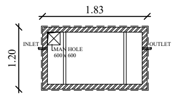
FOUNDATION DETAIL
