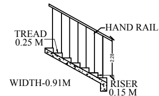
STAIRCASE DETAILS
