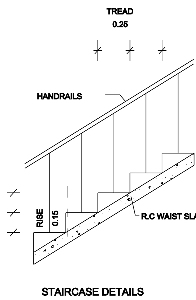
STAIRCASE DETAILS
