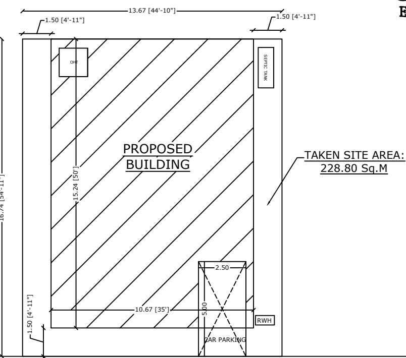
TAKEN SITE PLAN:- (SCALE 1:100)
