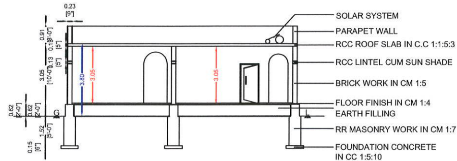
SECTION "AB"
