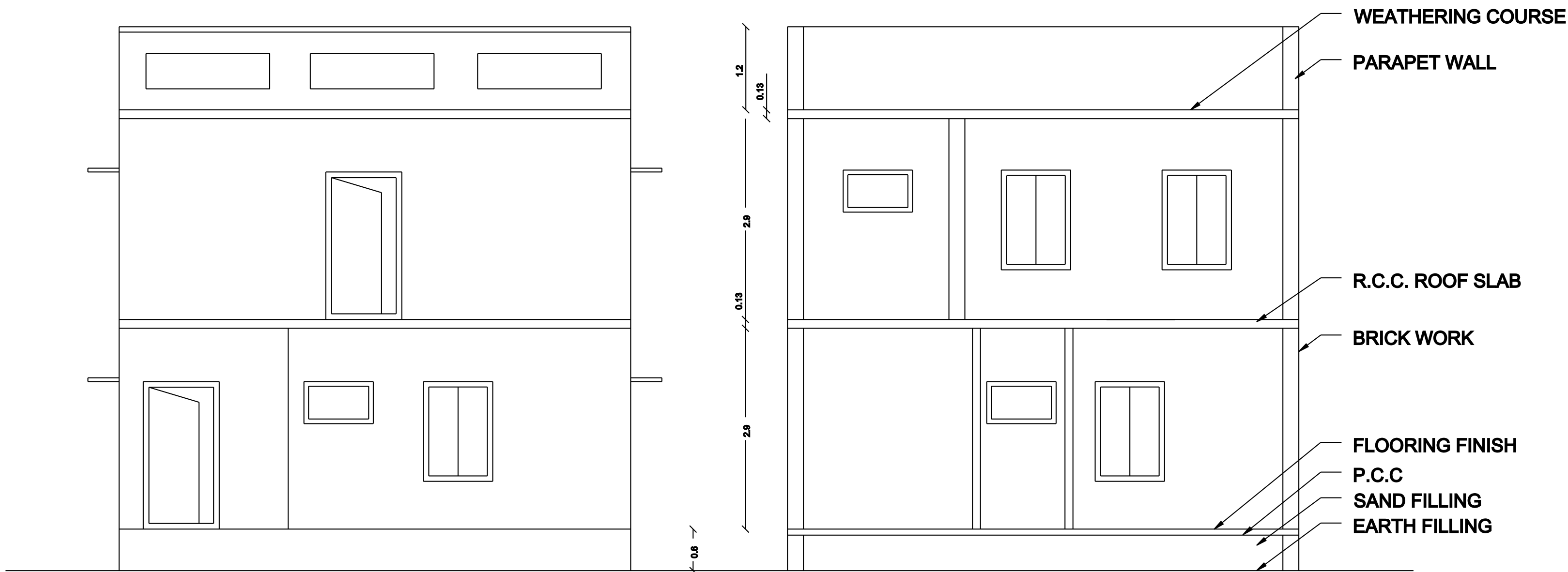
FRONT ELEVATION
