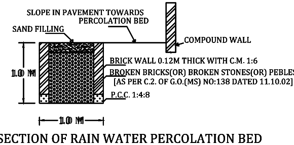
SECTION OF RAIN WATER PERCOLATION BED
