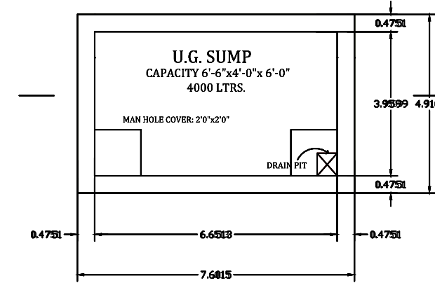
SUMP DETAIL SCALE 1"=4'0"
