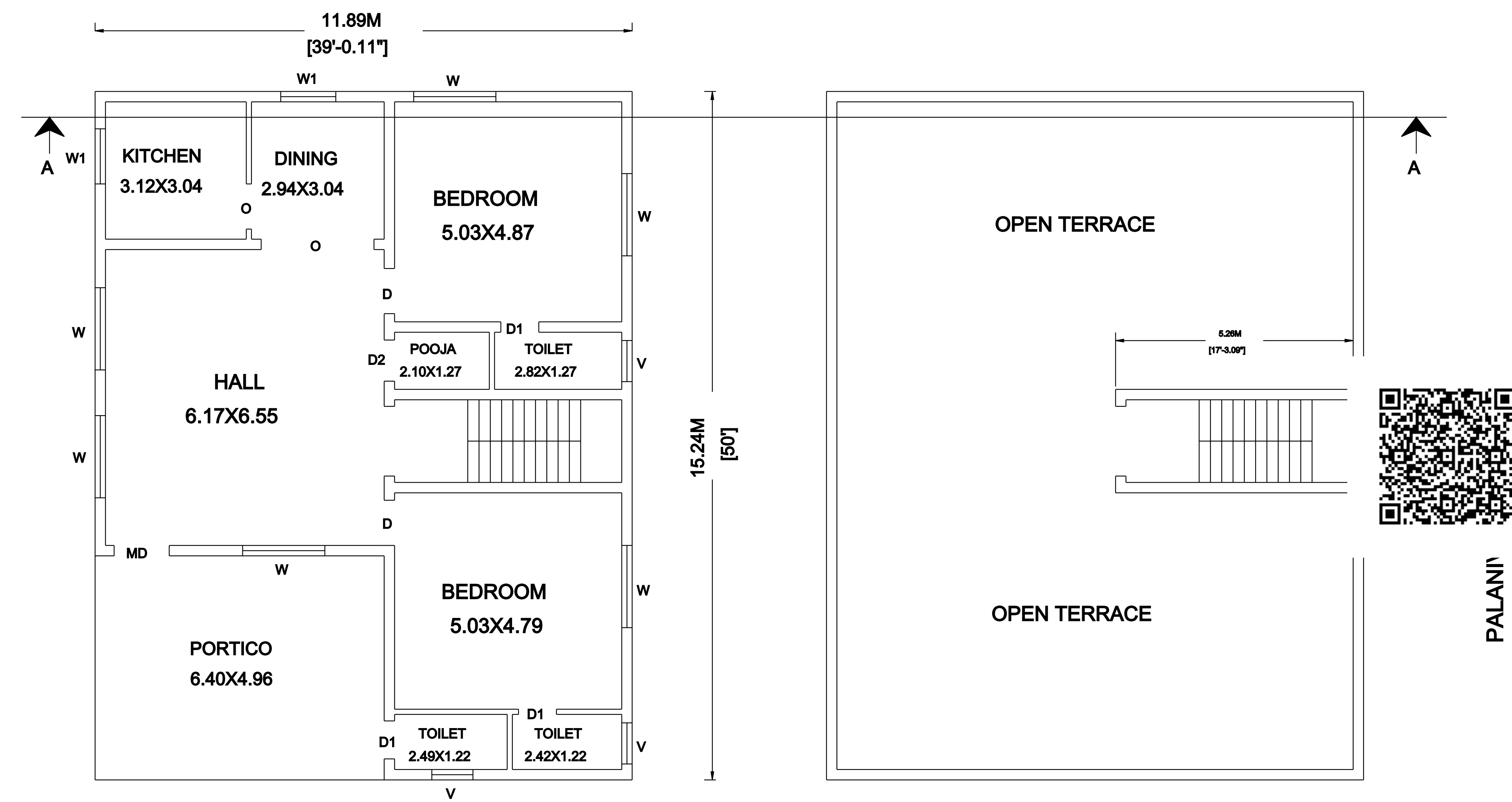
PRO.GROUND FLOOR PLAN
