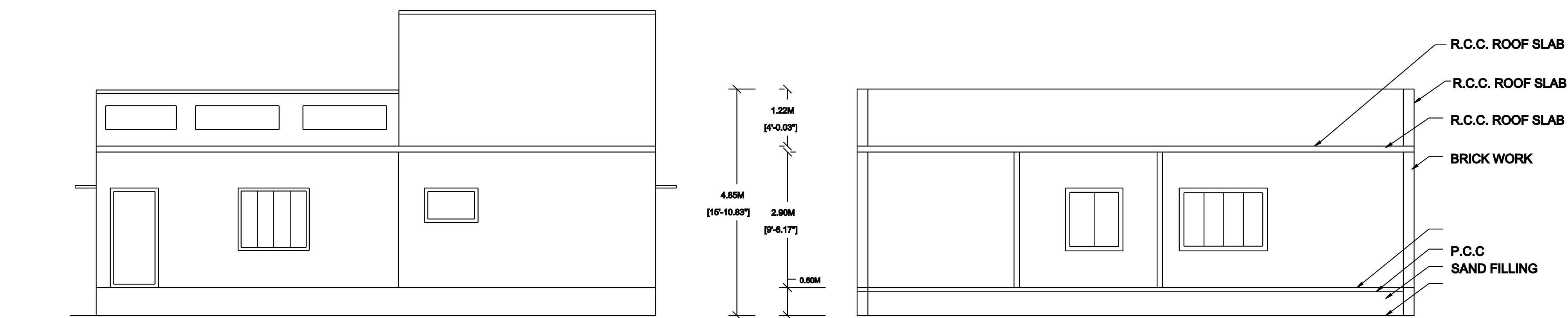
FRONT ELEVATION
